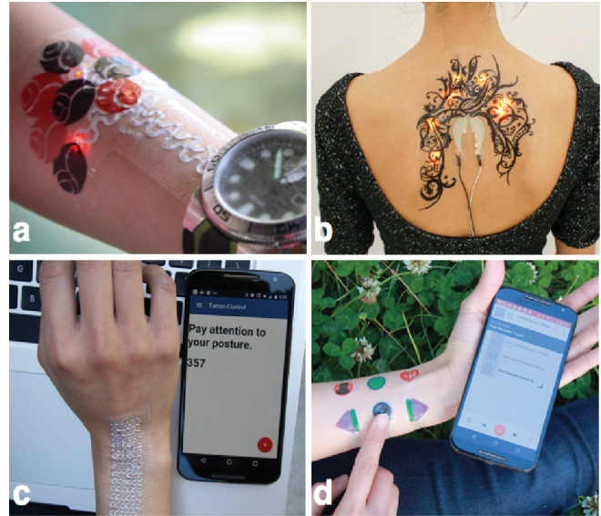
Figure 1. Skintillates is a class of temporary tattoo electronics that can be fabricated using an accessible process. a) A point-light display, b) A back tattoo LED display that flashes with music, c) A strain gauge that detects body position, d) capacitive buttons for mobile device control
